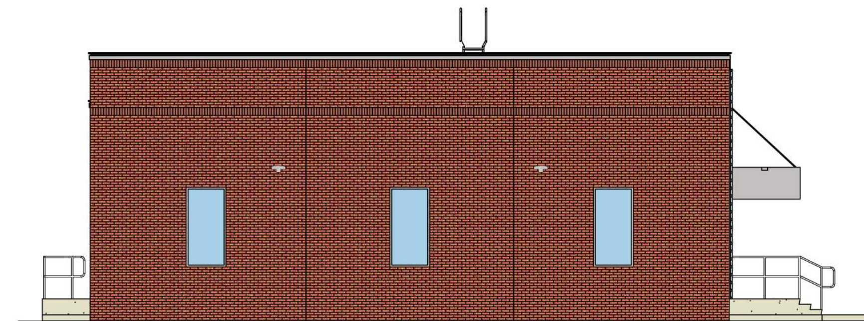
West Elevation
